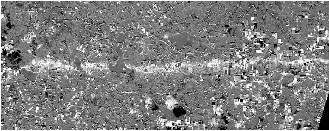
Figure 9(c): July 5 th (17 days after tornado) – Second PC using bands 1,2,5 and 7.
