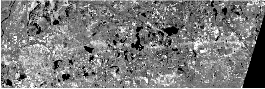
Figure 4(c): June 19, 2001 - Landsat ETM+, Band 5 (mid-infrared).
