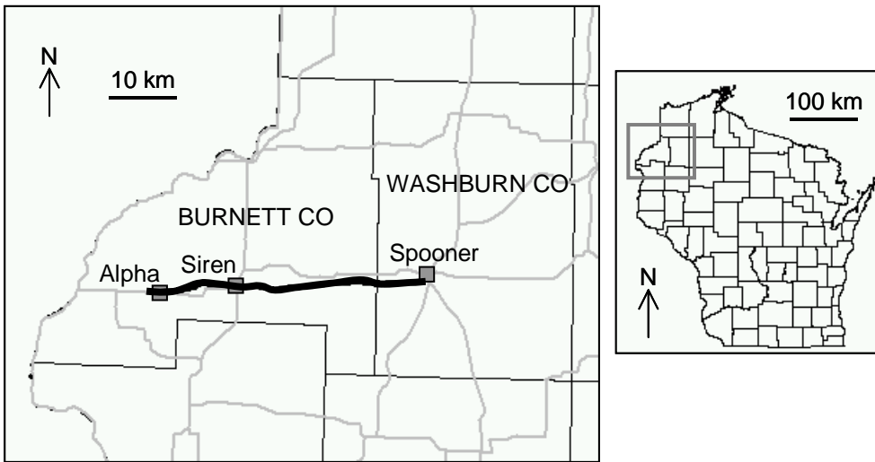
Figure 1. Map of Wisconsin showing the location of Burnett County and the approximate path of “The Siren Tornado.”
