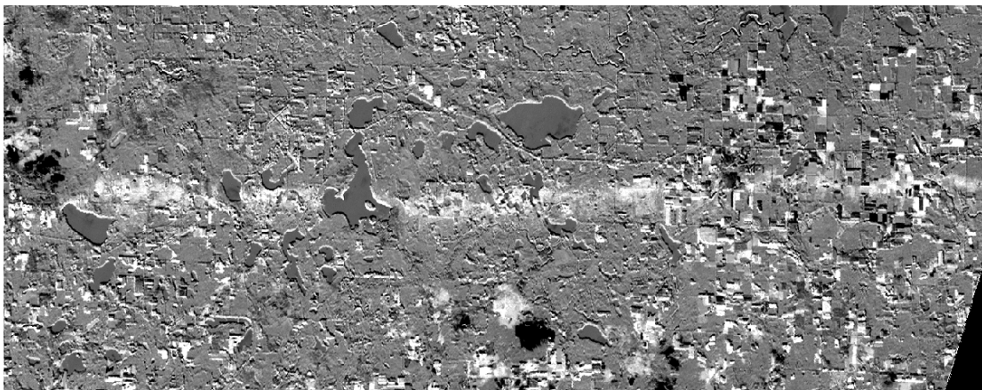
Figure 9(b): June 28 th (10 days after tornado) – Second PC using bands 1,2,5 and 7.
