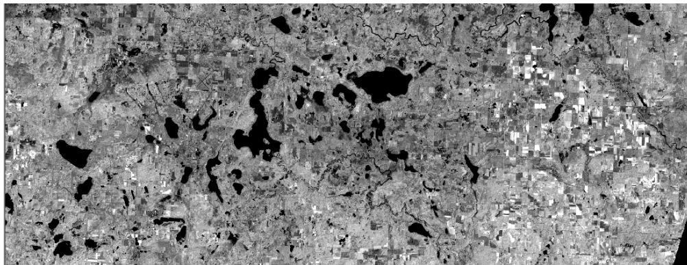
Figure 6: June 19, 2001 – Panchromatic band, 15 meter spatial resolution.
