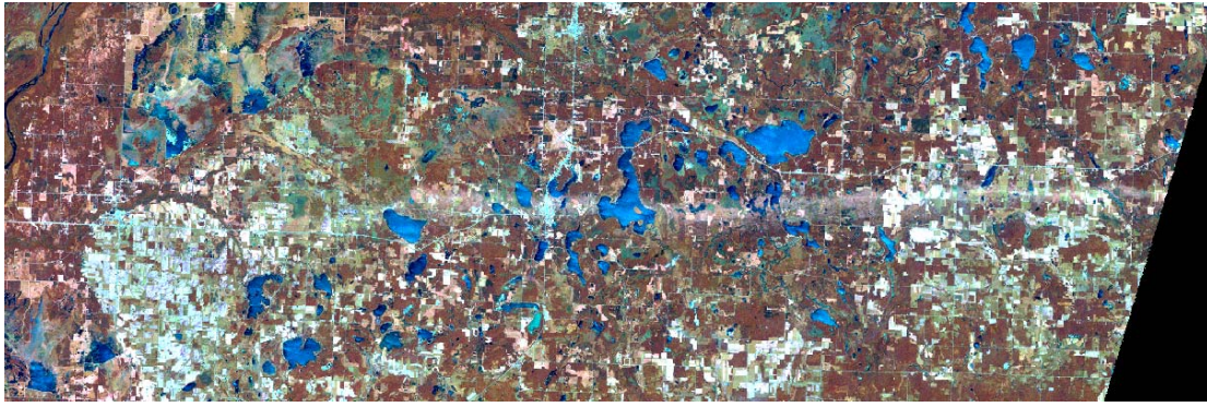
Figure 5(c): June 19, 2001 – Color Composite (red - band 5, green - band 3, blue – band 2).
