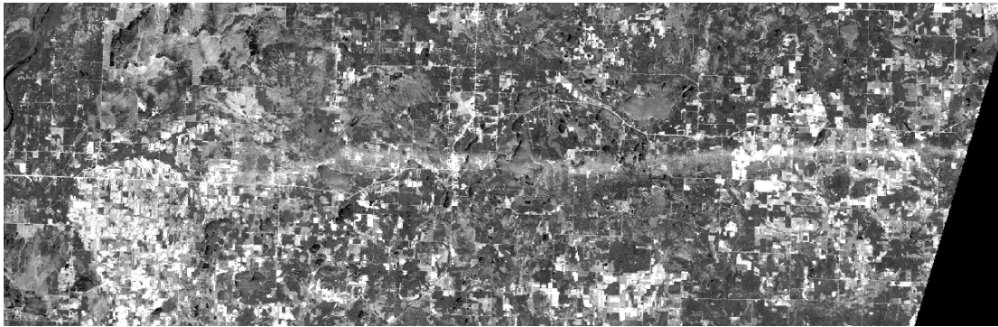
Figure 4(a): June 19, 2001 (1 day after tornado) - Landsat ETM+, Band 2 (green).
