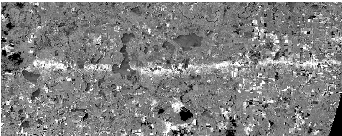
Figure 9(a): June 19 th (1 day after tornado) – Second PC using bands 1,2,5 and 7.
