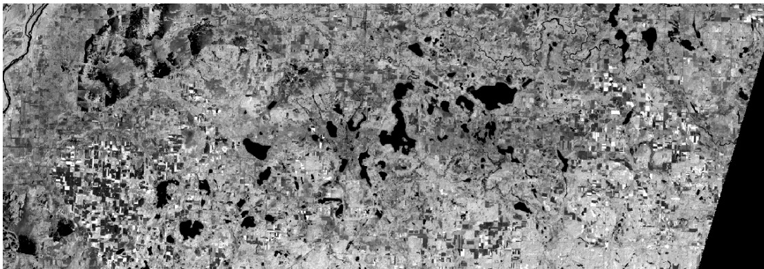
Figure 4(b): June 19, 2001 - Landsat ETM+, Band 4 (near-infrared).
