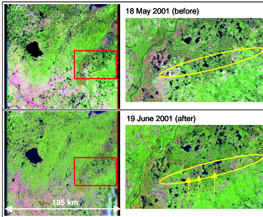
Figure 3. “Before” (May 18, 2001) and “After” (June 19, 2001) browse images of the tornado damage track.
