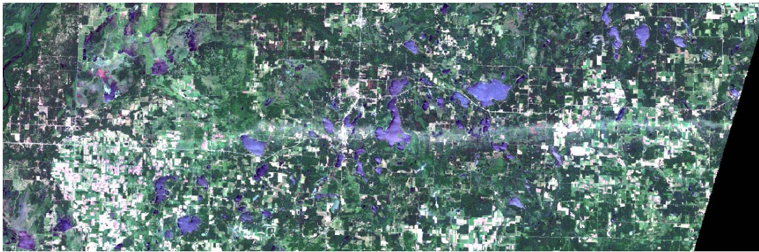
Figure 5(a): June 19, 2001 – Color Composite (red-band 3, green - band 2, blue – band 1).
